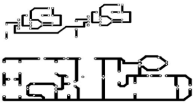
Figure 7. PCB Design done in Diptrace Software
