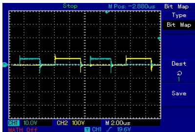
Figure 8. Pulse Output from PIC 16F877A
