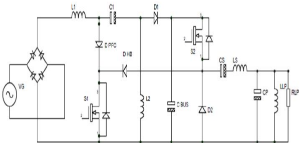
Figure 1. Proposed Single-Stage SEPIC Half-Bridge Integrated electronic Ballast
