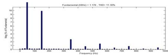
Figure 6. THD Measured in Input Current Waveform
