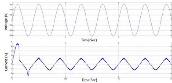
Figure 5. Input Current and Voltage Waveforms
