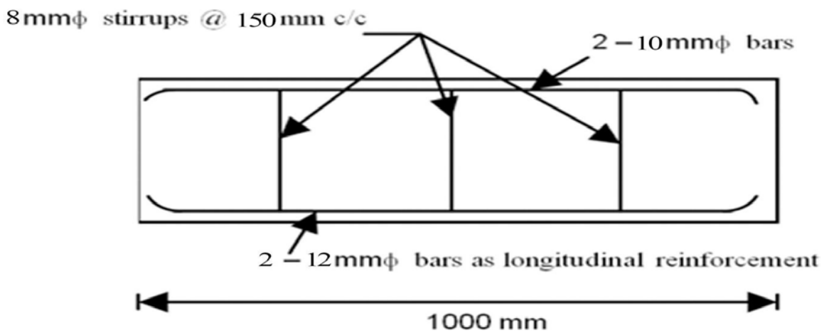
Fig 1 Reinforcement detailing of the beam
