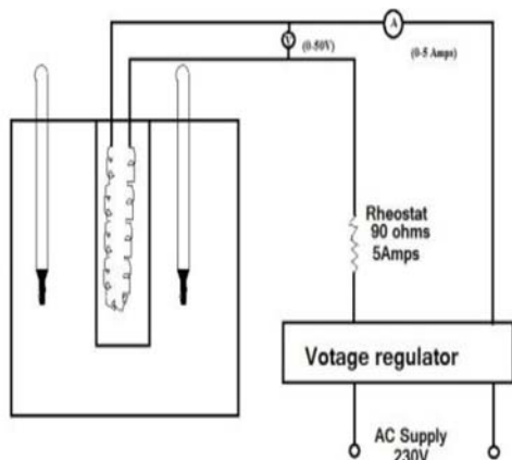
Figure 5: Schematic Diagrams for Experimental Measuring Instruments
