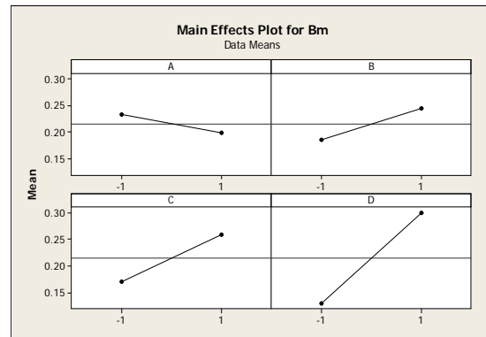
Figure 6: Main Effect for Heat Accumulation Factor
