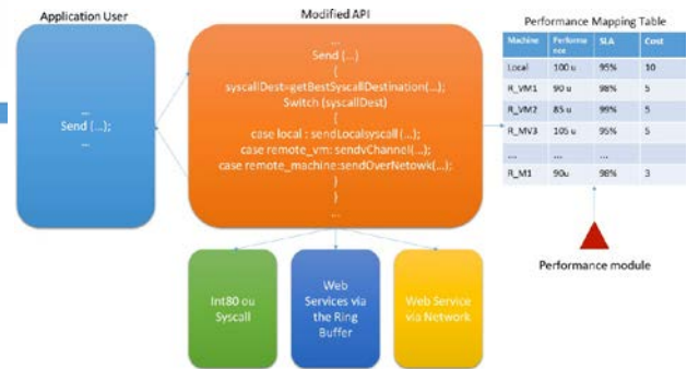
Fig. 5. Syscalls routines dispatching system based on business rules
