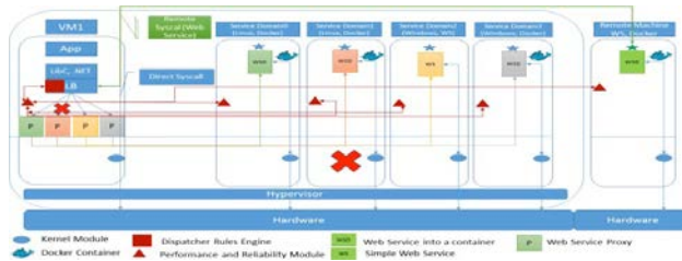
Fig. 4. Syscalls processing
