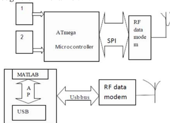
Fig 3.1: Block diagram
