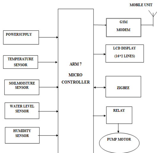
Fig: 1:Block diagram Transmitter section
