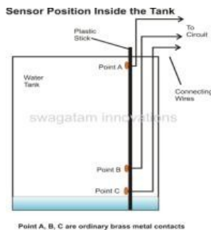
FIG: 7: WATER LEVEL SENSOR
