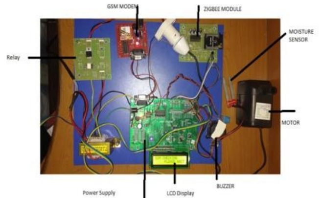
Fig: 11: Transmitter section
