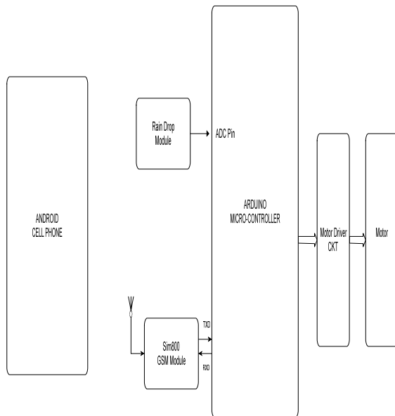
Figure.1 Block diagram
