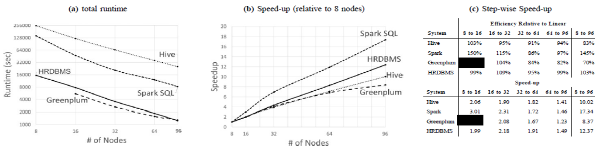
Fig. 7: 1TB TPC-H experiments: (a) total runtime, (b) speed-up relative to 8 nodes, and (c) step-wise speed-up
