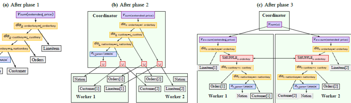
Fig. 6: Optimizing the query from Example 1. We show the query plan after each optimization phase.
