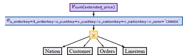
Fig. 5: Initial plan for the query from Example 1
