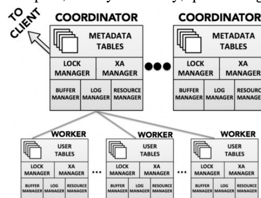
Fig. 1: Anatomy of a HRDBMS cluster
