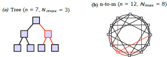
Fig. 4: Exemplary tree and n-to-m topologies
