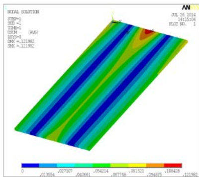
Fig.15 Displacement Plot
