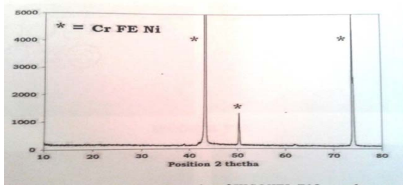
Fig.11 Showing XRD peaks of INCONEL-718
