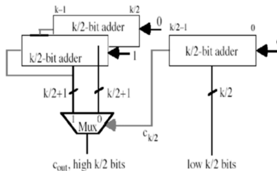
Fig. 2 Block diagram of k-bit adder
