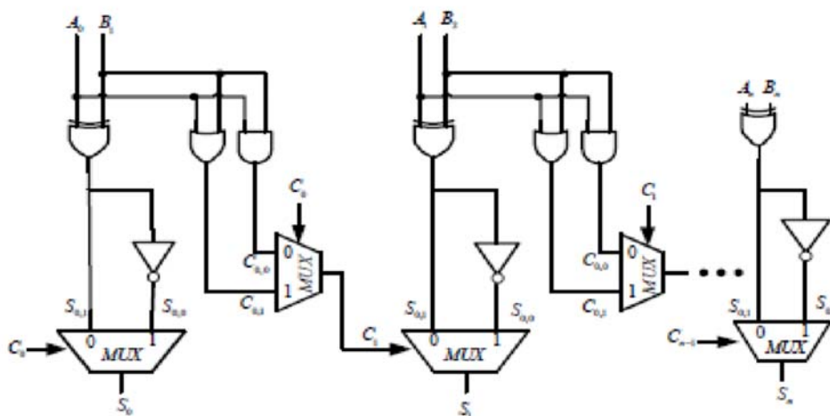
Fig. 5 Internal structure of the proposed area-efficient carry select adder is constructed by sharing the common
