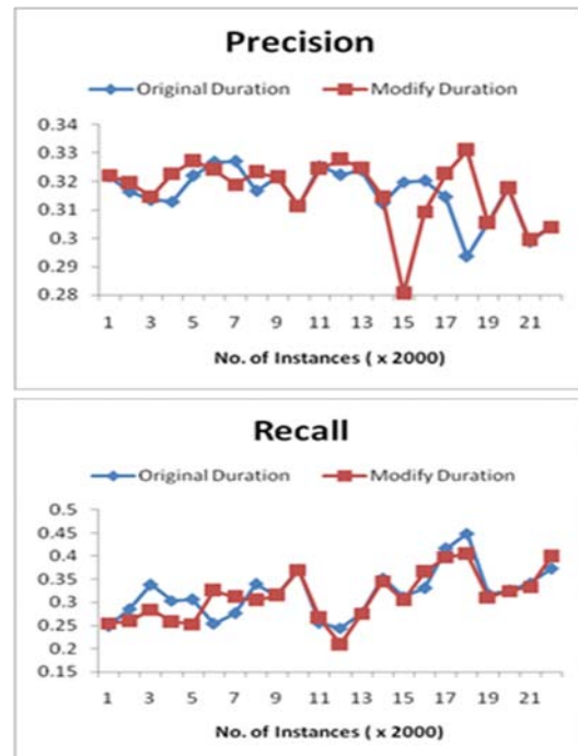
Figure 4.9: Accuracy on attribute Duration in Bank Management with 5-Cluster
