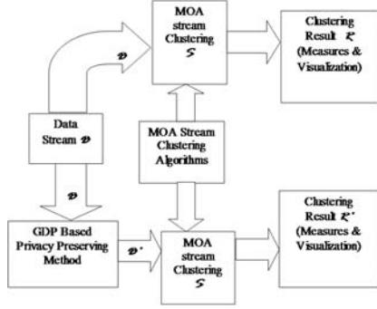
Figure.1 Framework for privacy preserving using clustering
