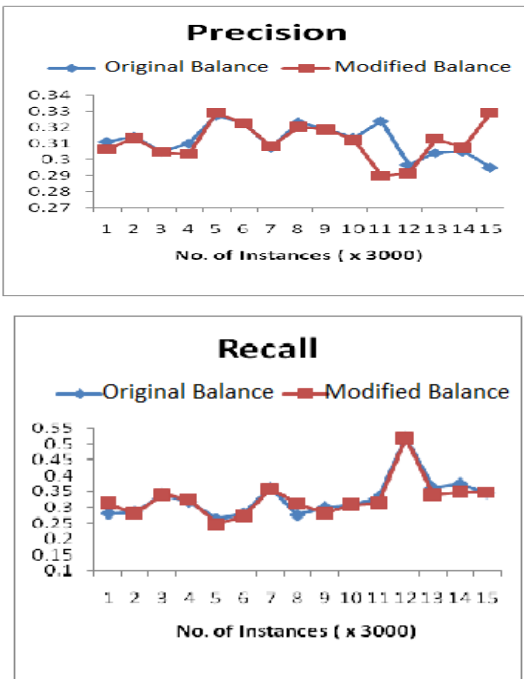
Figure 4.11: Accuracy on attribute Balance in Bank Management with 5-Cluster
