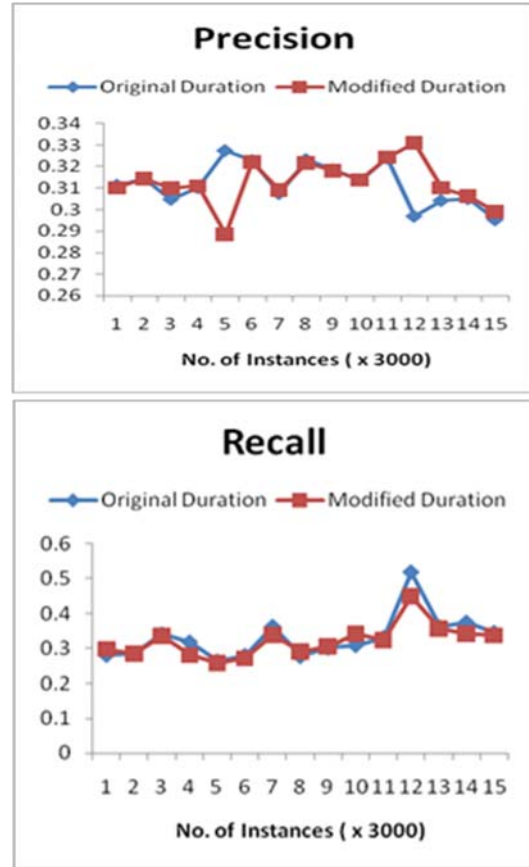
Figure 4.12: Accuracy on attribute Duration in Bank Management with 5-Cluster
