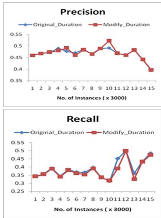
Figure 4.18: Accuracy on attribute Duration in Bank Management with 3-Cluster
