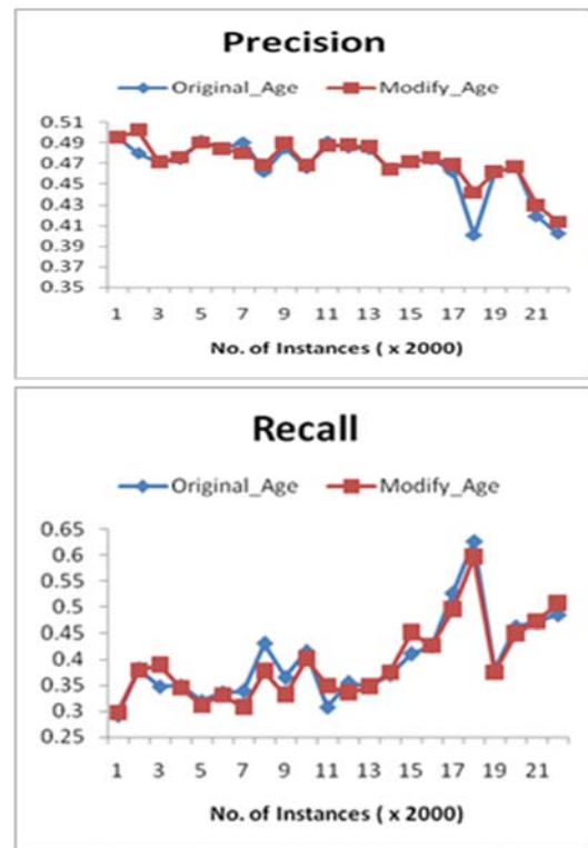
Figure 4.13: Accuracy on attribute Age in Bank Management with 3-Cluster
